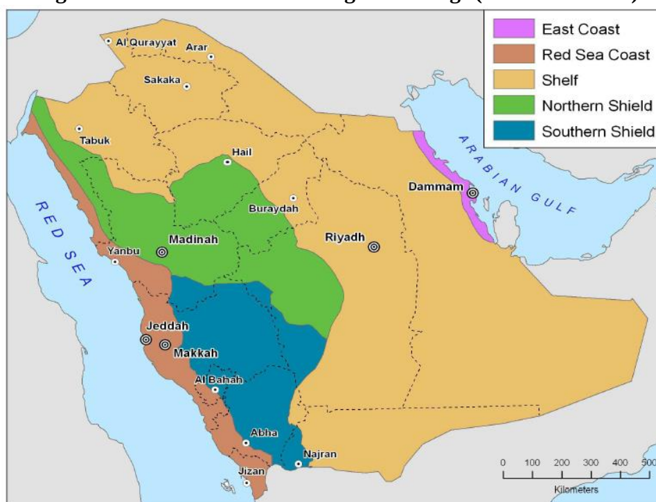
Figure 1.1: Saudi Arabian Geological Settings (AlTokhais 2018)
